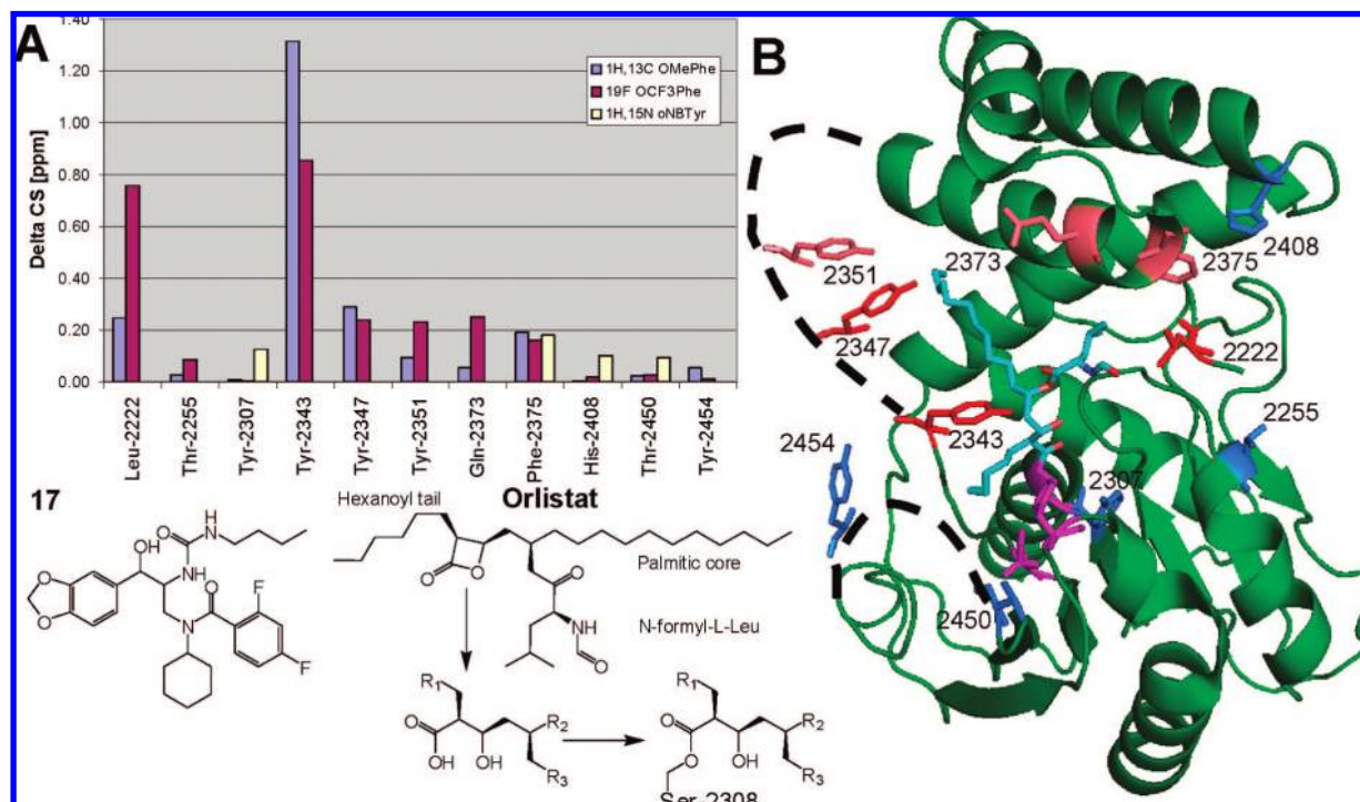
Figure 8. Chemical shift mapping of tool compound 17 binding to FAS-TE. (A) Combined chemical shift data. Chemical shift changes \Delta CS of ^{19}\text{F} resonances (OCF 3 Phe; purple) were scaled relative to ^1\text{H} by the gyromagnetic ratio while ^1\text{H} - ^{13}\text{C} (OMePhe; violet) and ^1\text{H} - ^{15}\text{N} (oNBtyr; pale yellow) chemical shifts were combined using the expression \Delta\text{CS} = [(\Delta^1\text{H})^2 + (0.252 \cdot \Delta^{13}\text{C})^2]^{0.5} and \Delta\text{CS} = [(\Delta^1\text{H})^2 + (0.102 \cdot \Delta^{15}\text{N})^2]^{0.5} , respectively. OMePhe and OCF 3 Phe at Tyr-2307 block binding (see text). For oNBtyr mutants only a limited set of chemical shift changes could be compiled because of conformational exchange (see text). (B) Structure of the covalent orlistat complex (2PX6.pdb). 30 The average chemical shift changes induced by the binding of 17 are calculated for each unnatural amino acid and color-coded for each position: \Delta\text{CS} < 0.1 ppm, blue; 0.1 – 0.2 ppm, salmon; > 0.2 ppm, red. Disordered loops are indicated by dashed lines. The active site residues Ser-2308, Asp-2338, and His-2481 are shown in magenta.
